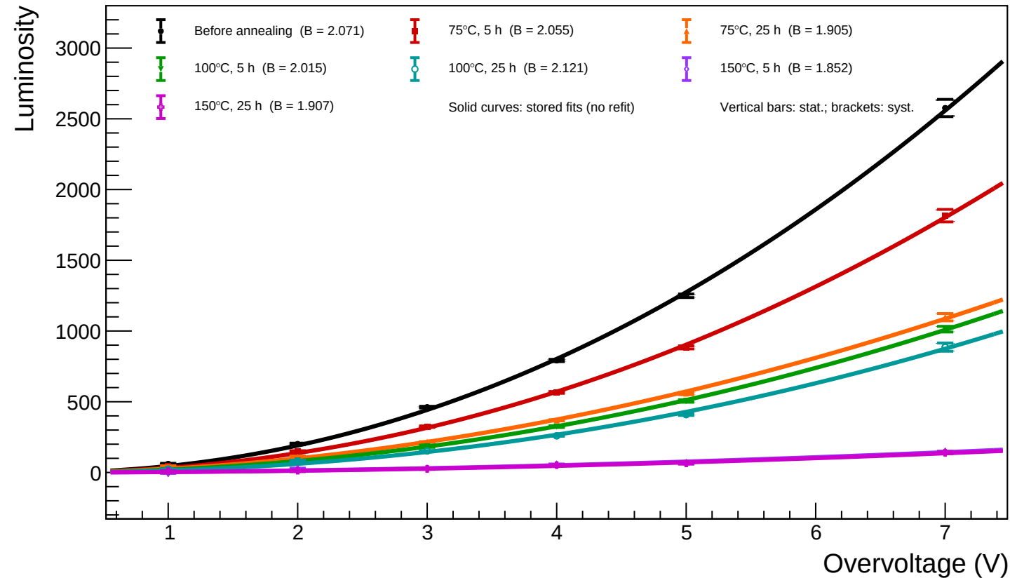
A1_T=20 - Spot 13 ( x = 429.64 , y = 487.00 ): luminosity vs overvoltage for all annealing phases
