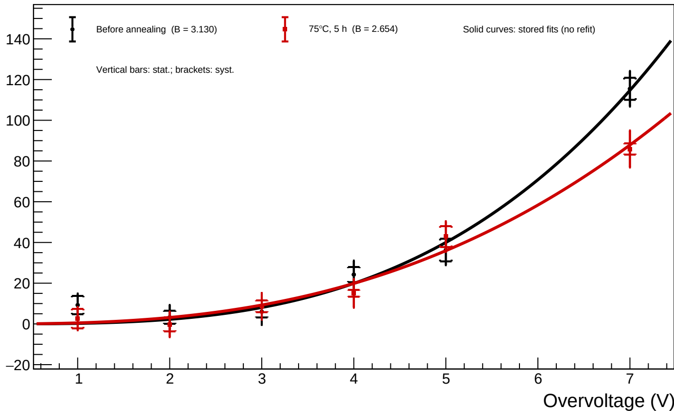
A1_T=20 - Spot 15 ( x = 596.49 , y = 527.90 ): luminosity vs overvoltage for all annealing phases
