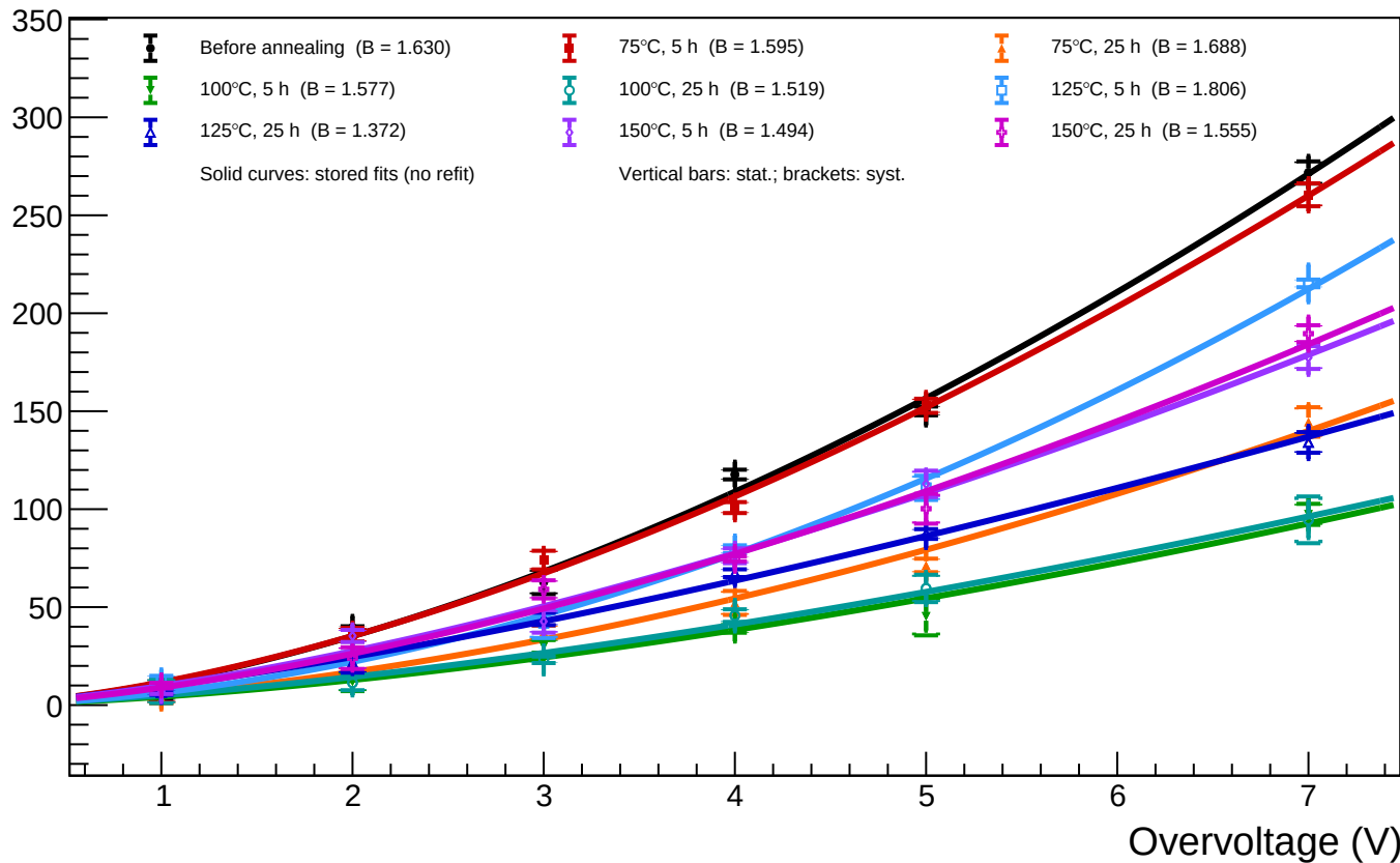
A1_T=20 - Spot 17 ( x = 649.48 , y = 440.37 ): luminosity vs overvoltage for all annealing phases
