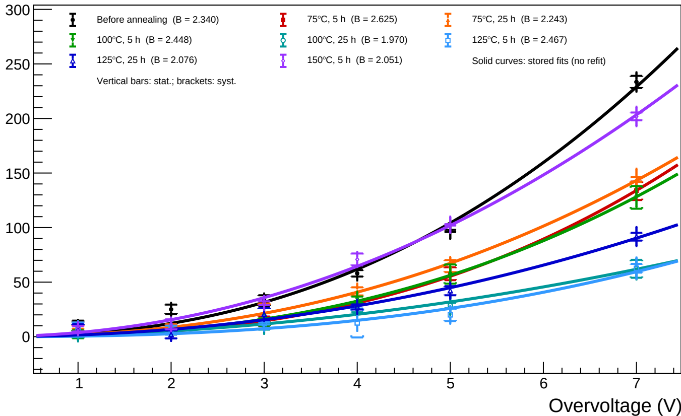
A1_T=20 - Spot 19 (x = 660.82, y = 688.43): luminosity vs overvoltage for all annealing phases
