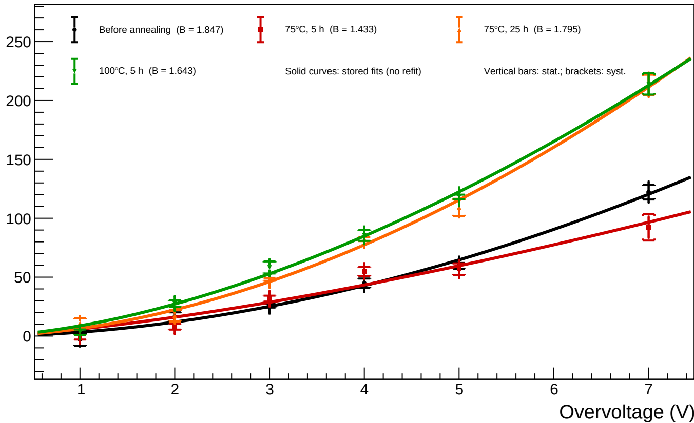
A1_T=20 - Spot 2 (x = 139.66, y = 257.62): luminosity vs overvoltage for all annealing phases
