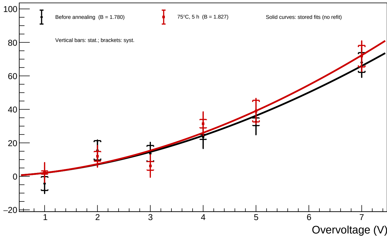
A1_T=20 - Spot 20 ( x = 700.54 , y = 366.46 ): luminosity vs overvoltage for all annealing phases
