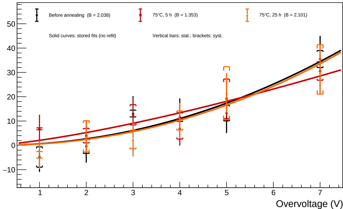
A1_T=20 - Spot 21 ( x = 739.68 , y = 314.35 ): luminosity vs overvoltage for all annealing phases
