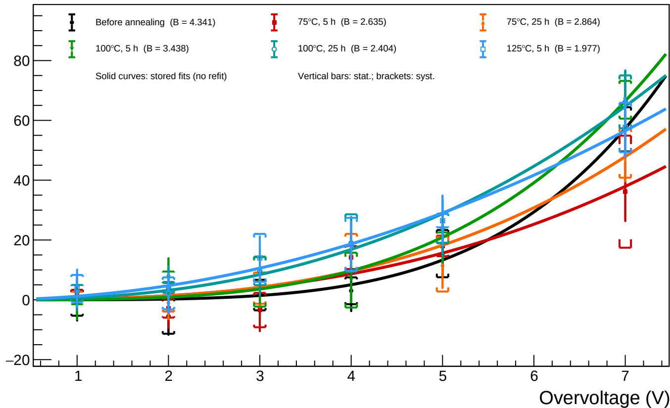
A1_T=20 - Spot 25 ( x = 872.05 , y = 566.97 ): luminosity vs overvoltage for all annealing phases
