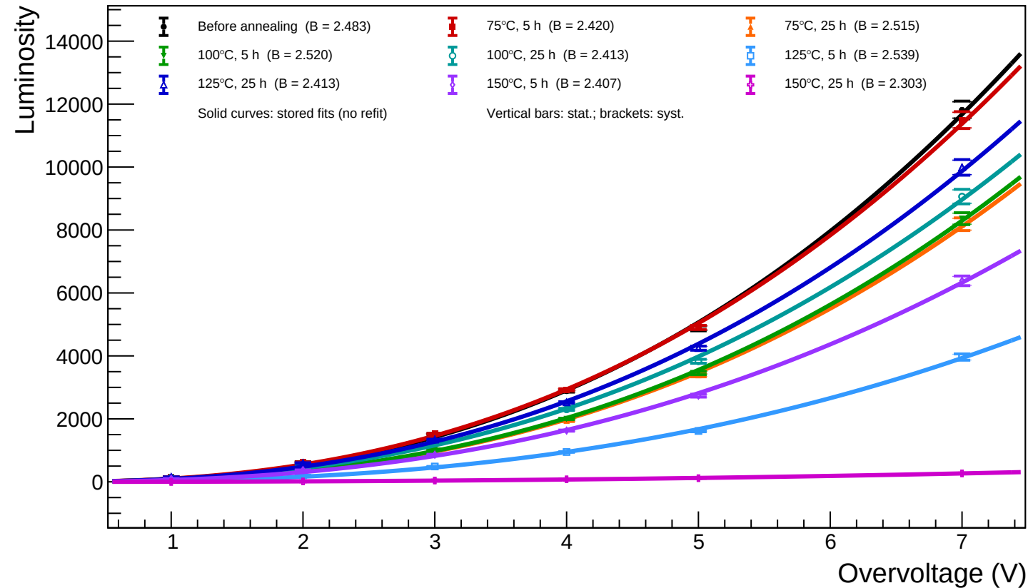
A1_T=20 - Spot 3 (x = 182.59, y = 172.15): luminosity vs overvoltage for all annealing phases
