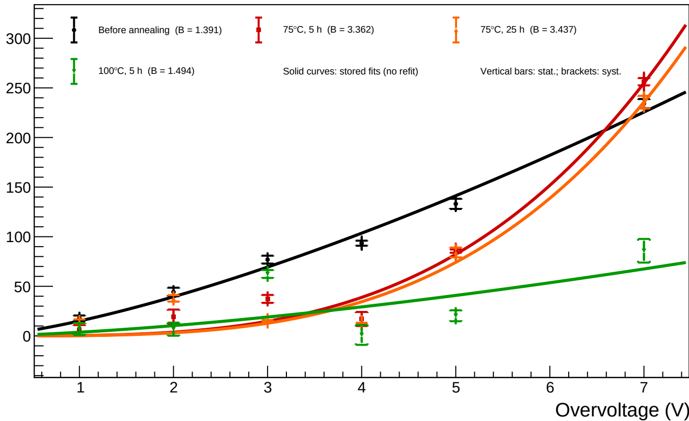
A1_T=20 - Spot 30 (x = 1088.01, y = 910.26): luminosity vs overvoltage for all annealing phases
