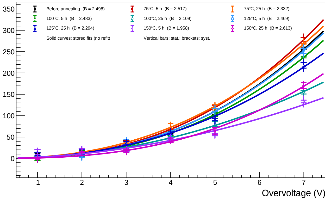
A1_T=20 - Spot 31 (x = 1089.04, y = 687.69): luminosity vs overvoltage for all annealing phases
