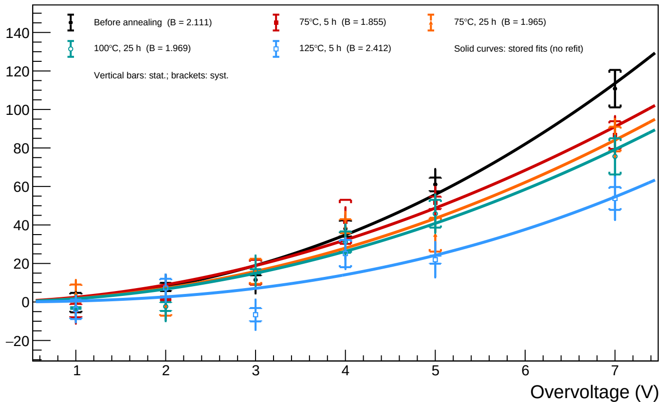
A1_T=20 - Spot 36 (x = 1241.46, y = 154.51): luminosity vs overvoltage for all annealing phases
