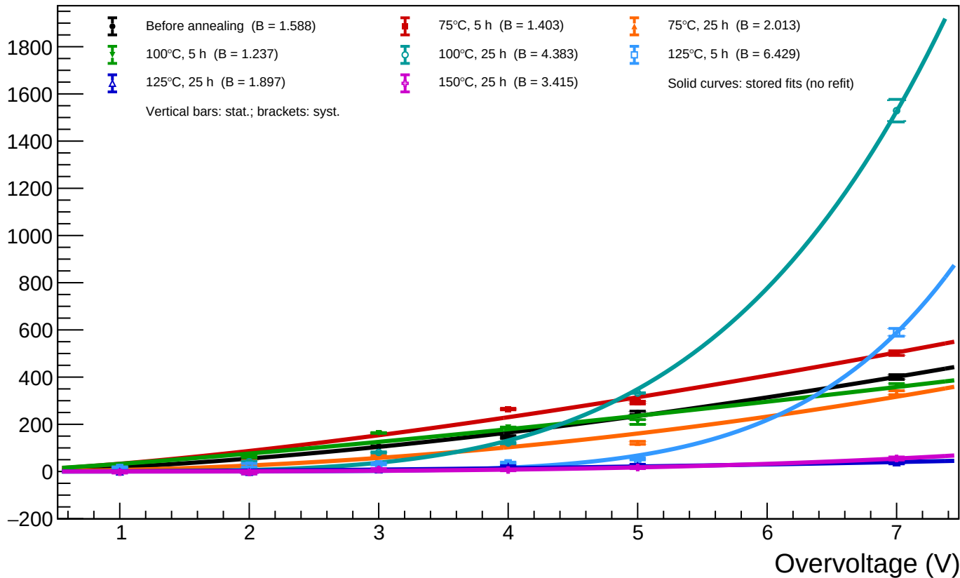
A1_T=20 - Spot 37 (x = 1244.59, y = 484.33): luminosity vs overvoltage for all annealing phases
