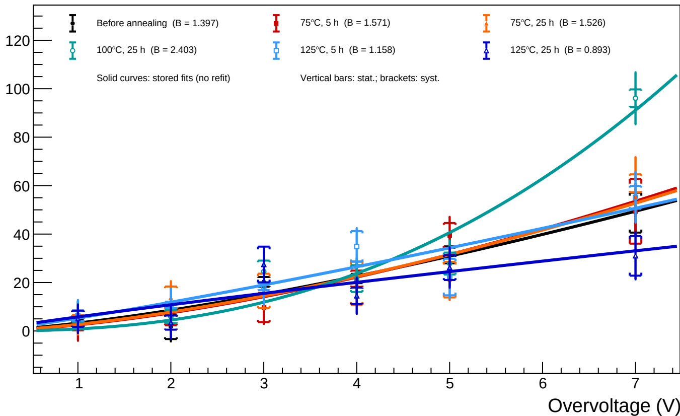
A1_T=20 - Spot 40 (x = 1266.92, y = 413.11): luminosity vs overvoltage for all annealing phases
