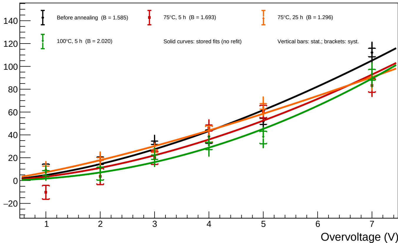
A1_T=20 - Spot 41 (x = 1287.85, y = 874.23): luminosity vs overvoltage for all annealing phases
