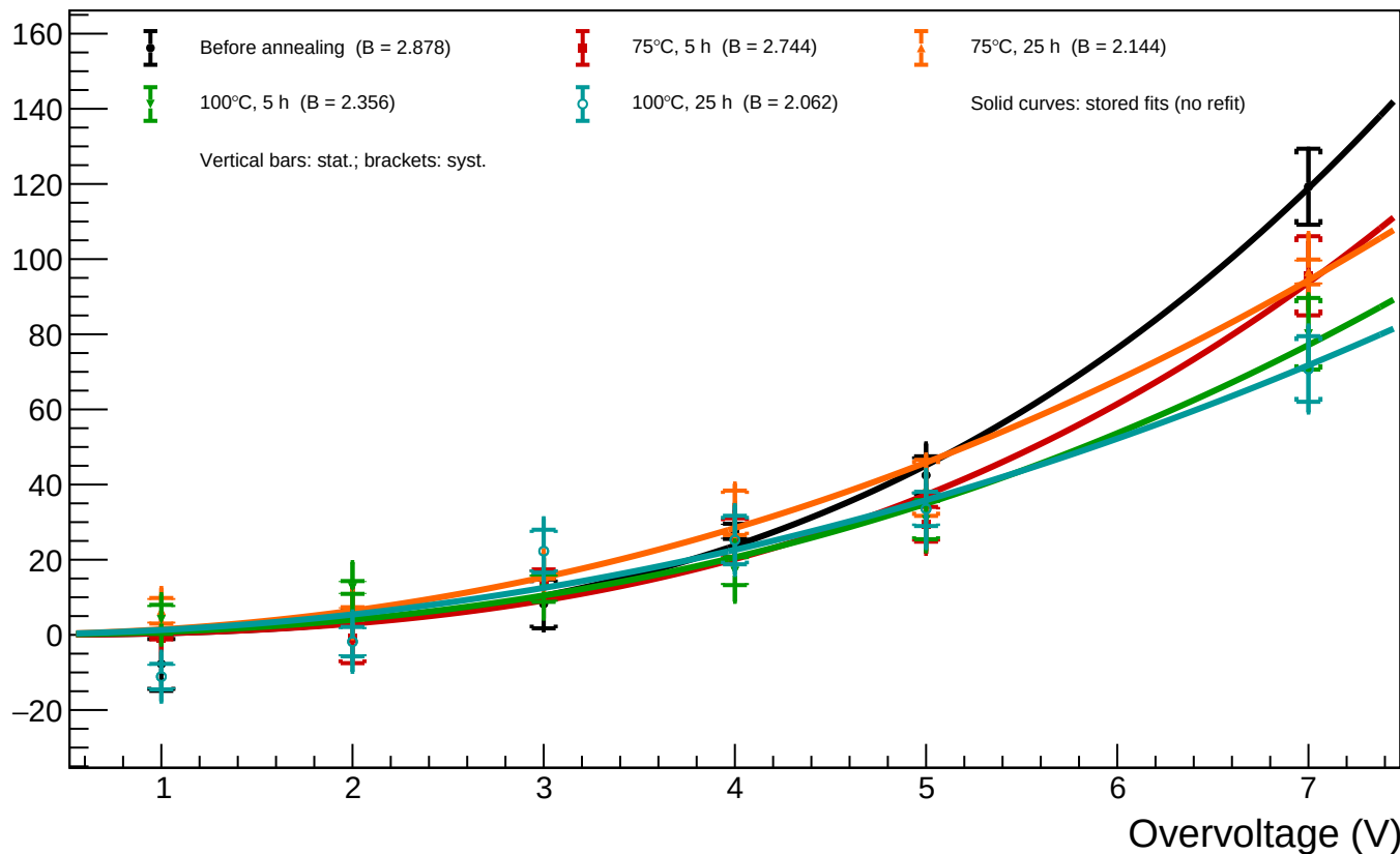
A1_T=20 - Spot 43 ( x = 1320.67 , y = 74.39 ): luminosity vs overvoltage for all annealing phases
