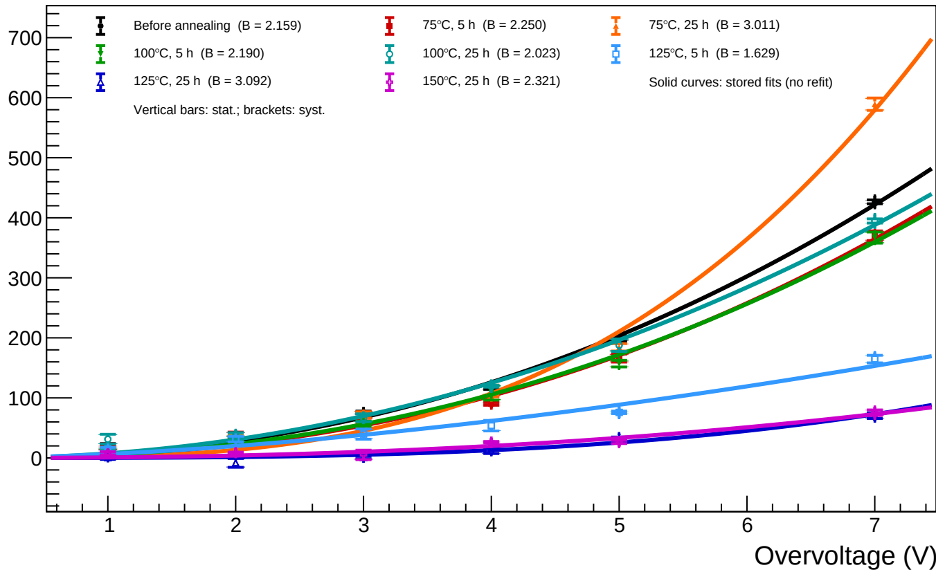
A1_T=20 - Spot 46 (x = 1376.04, y = 912.93): luminosity vs overvoltage for all annealing phases
