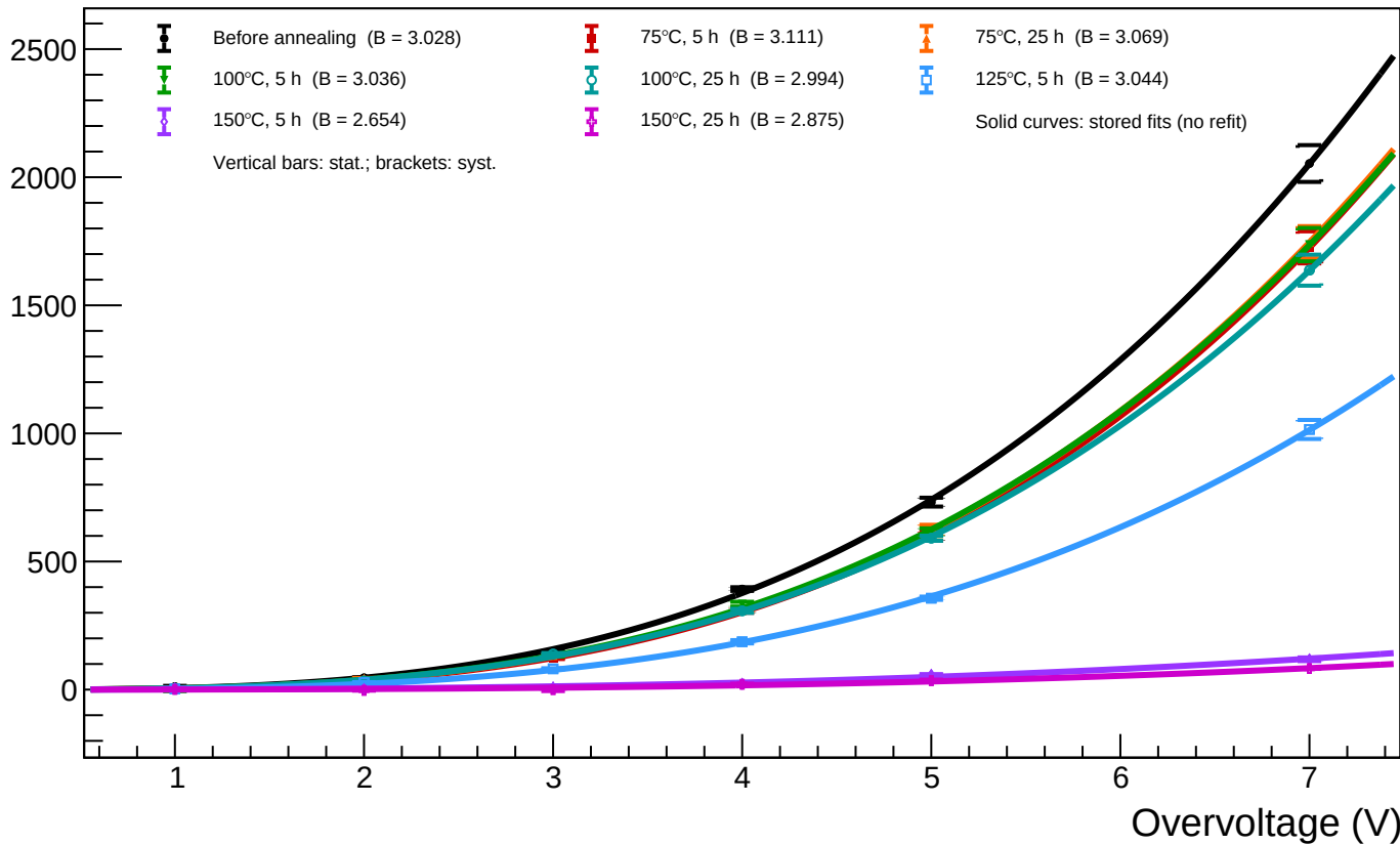
A1_T=20 - Spot 48 (x = 1497.05, y = 508.27): luminosity vs overvoltage for all annealing phases
