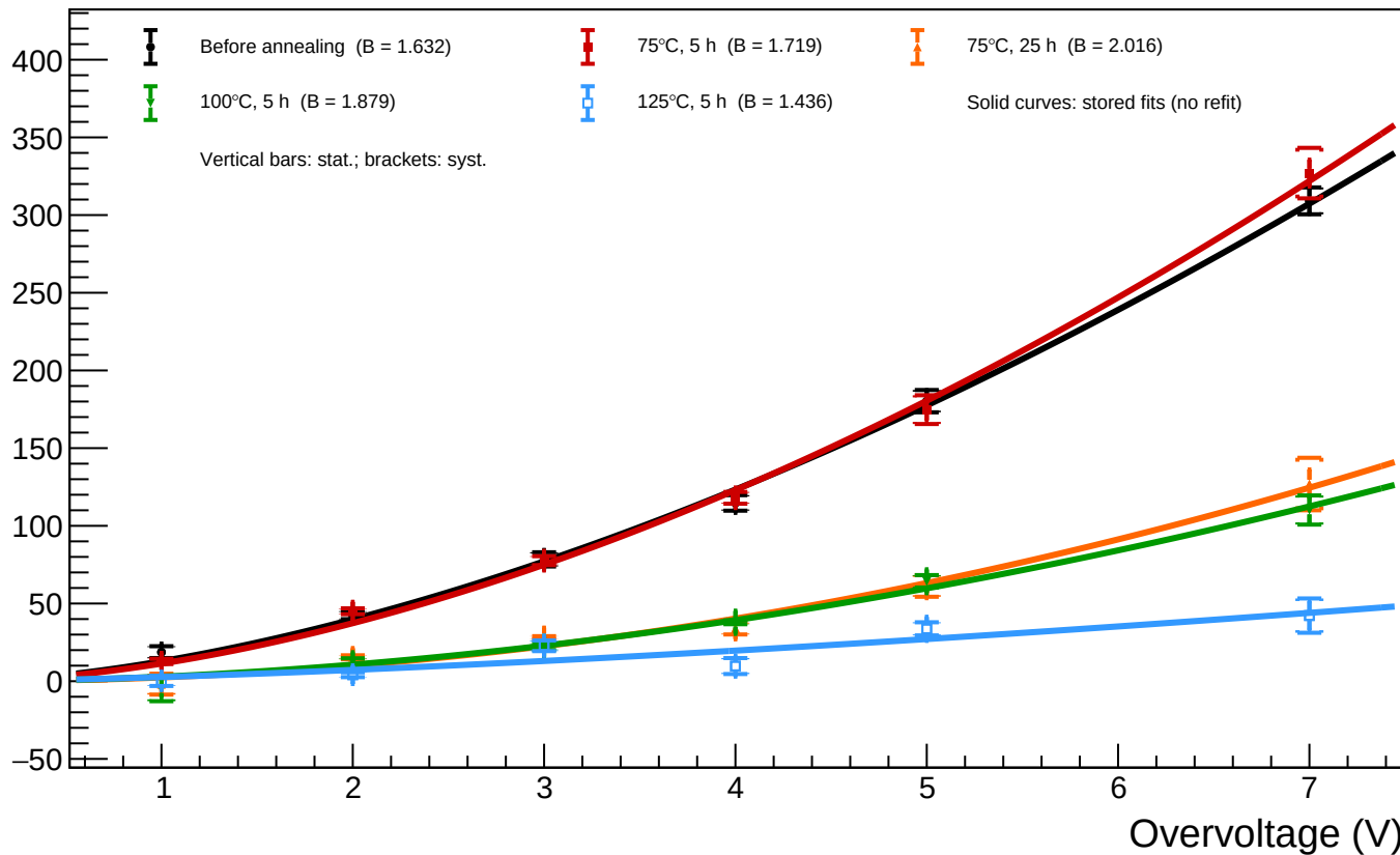
A1_T=20 - Spot 49 (x = 1502.80, y = 863.92): luminosity vs overvoltage for all annealing phases
