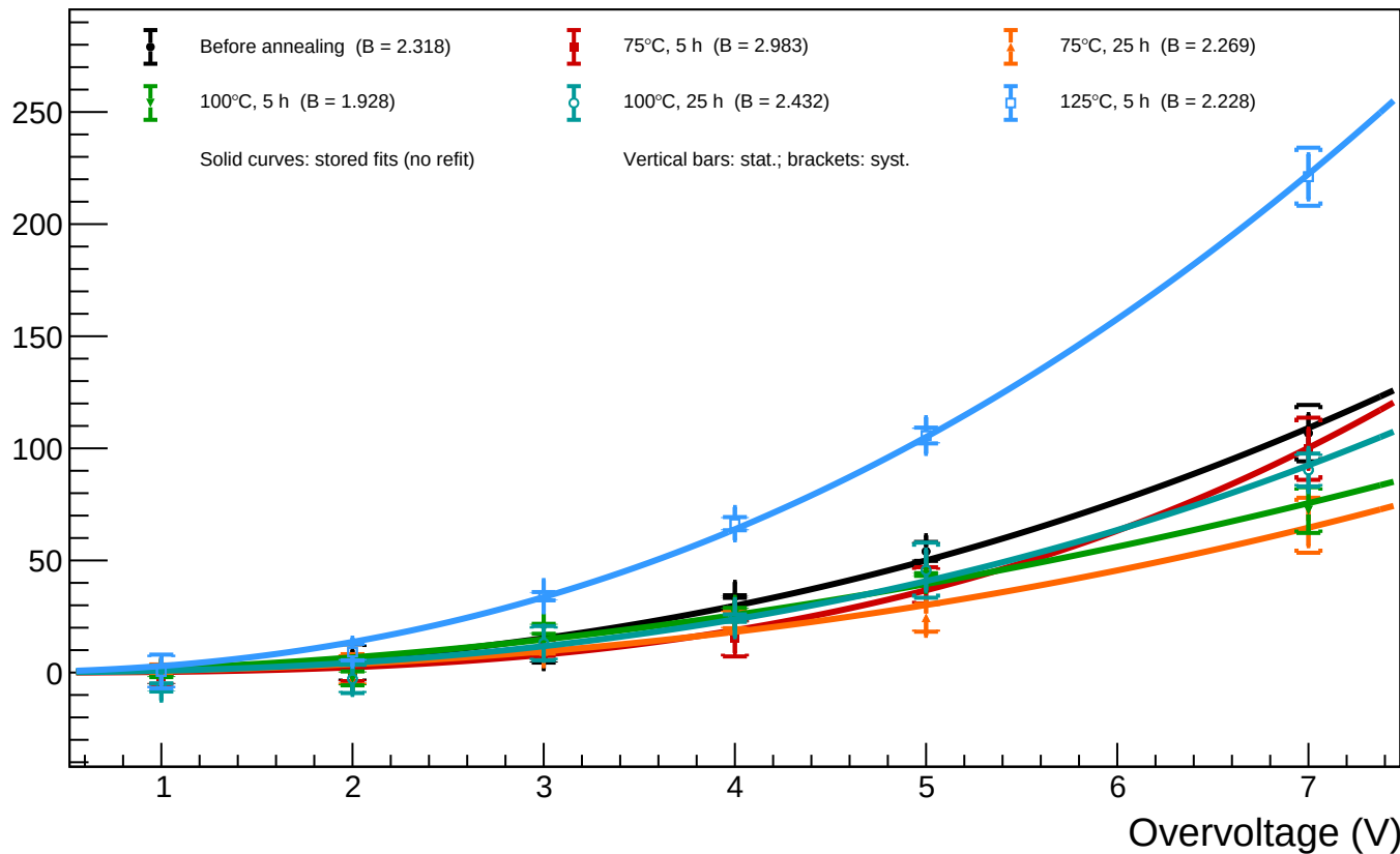
A1_T=20 - Spot 50 (x = 1536.40, y = 405.78): luminosity vs overvoltage for all annealing phases
