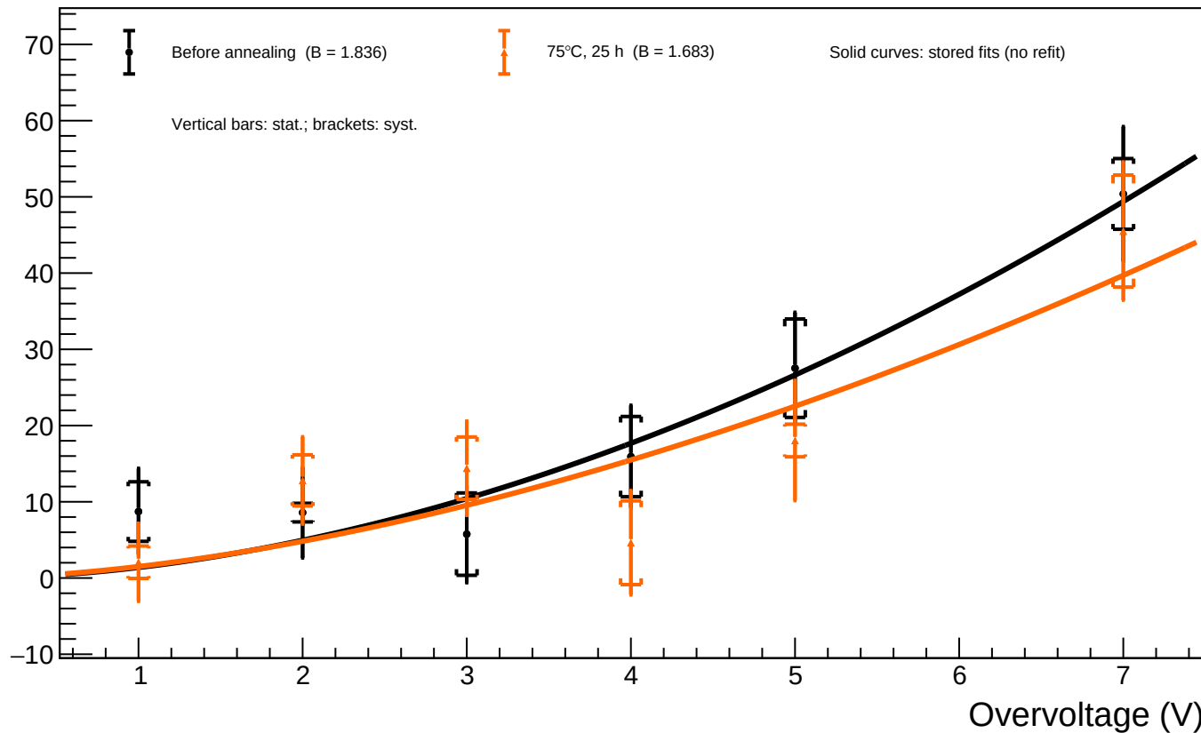
A1_T=20 - Spot 51 (x = 1584.70, y = 810.08): luminosity vs overvoltage for all annealing phases
