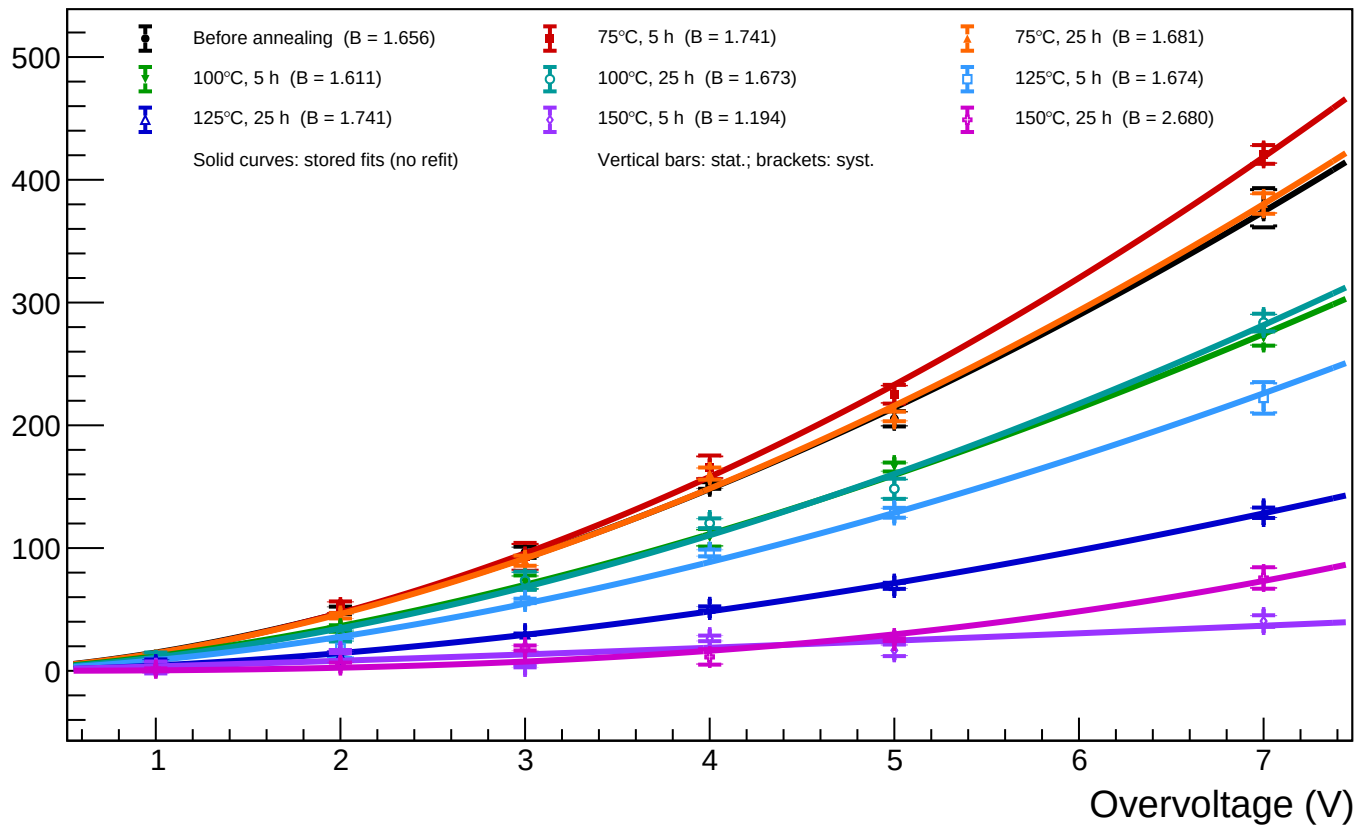
A1_T=20 - Spot 56 (x = 1782.75, y = 556.04): luminosity vs overvoltage for all annealing phases
