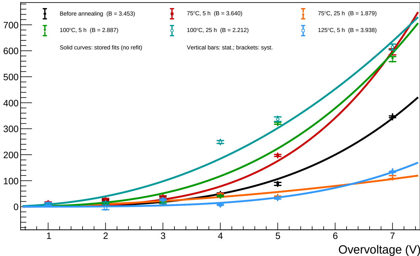
A1_T=20 - Spot 58 (x = 1821.57, y = 993.51): luminosity vs overvoltage for all annealing phases
