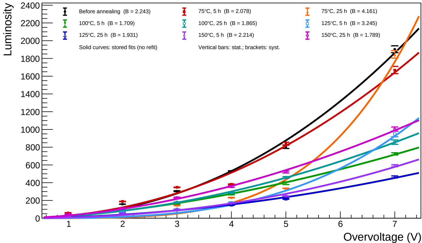
A1_T=20 - Spot 6 (x = 237.10, y = 244.17): luminosity vs overvoltage for all annealing phases
