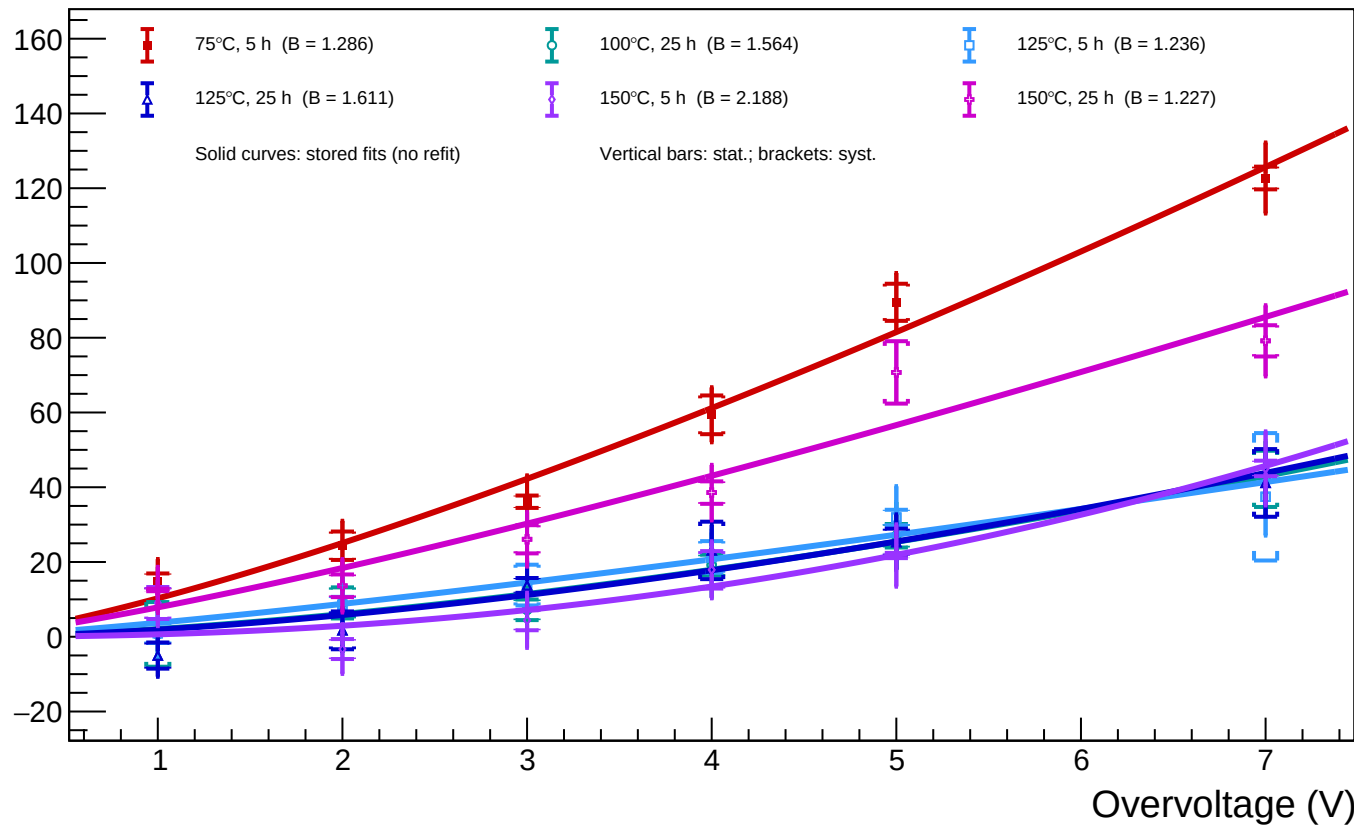
A1_T=20 - Spot 61 ( x = 454.66 , y = 766.63 ): luminosity vs overvoltage for all annealing phases
