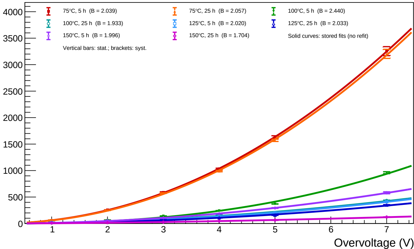
A1_T=20 - Spot 62 (x = 513.87, y = 881.63): luminosity vs overvoltage for all annealing phases
