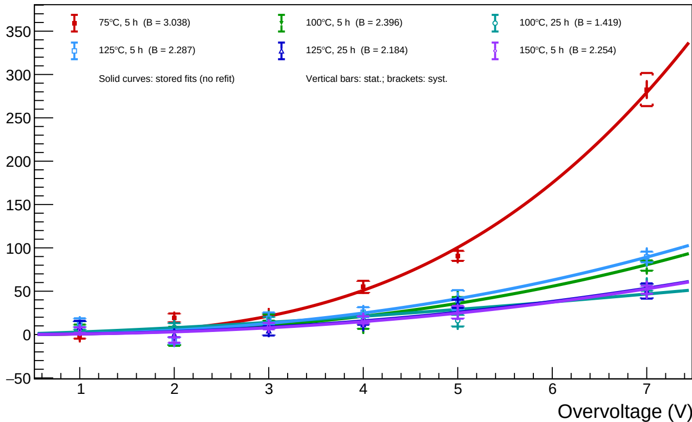
A1_T=20 - Spot 65 (x = 1176.15, y = 929.12): luminosity vs overvoltage for all annealing phases
