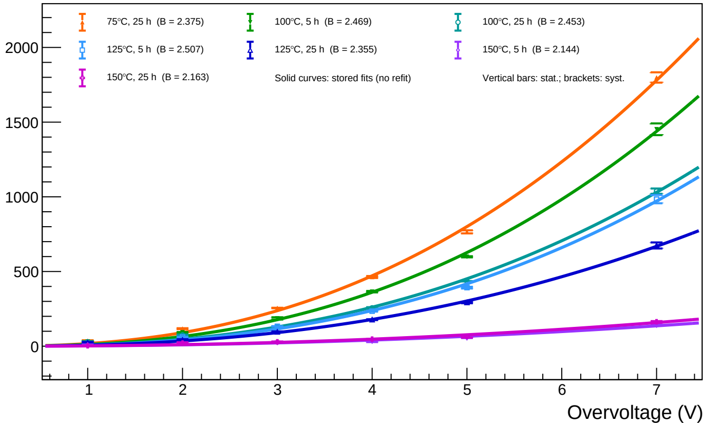
A1_T=20 - Spot 67 (x = 1616.34, y = 987.45): luminosity vs overvoltage for all annealing phases
