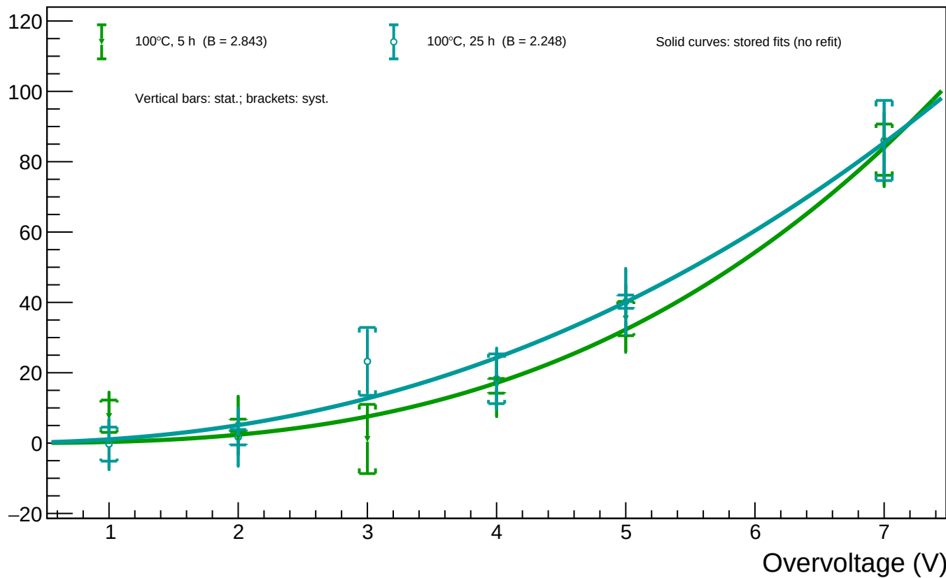
A1_T=20 - Spot 69 (x = 94.07, y = 353.22): luminosity vs overvoltage for all annealing phases
