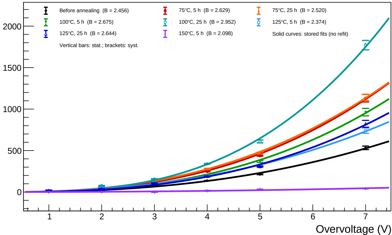
A1_T=20 - Spot 7 (x = 253.67, y = 351.34): luminosity vs overvoltage for all annealing phases
