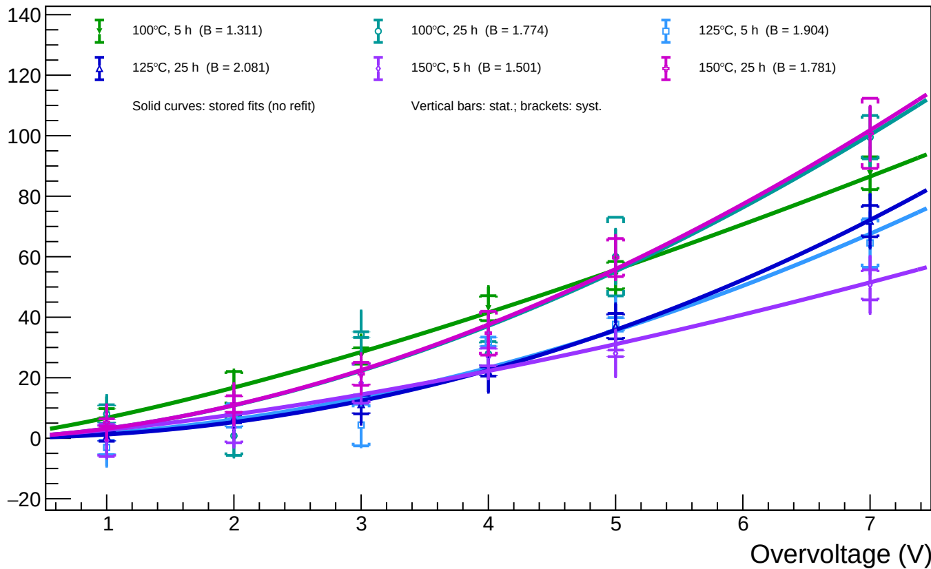
A1_T=20 - Spot 70 ( x = 336.36 , y = 286.80 ): luminosity vs overvoltage for all annealing phases
