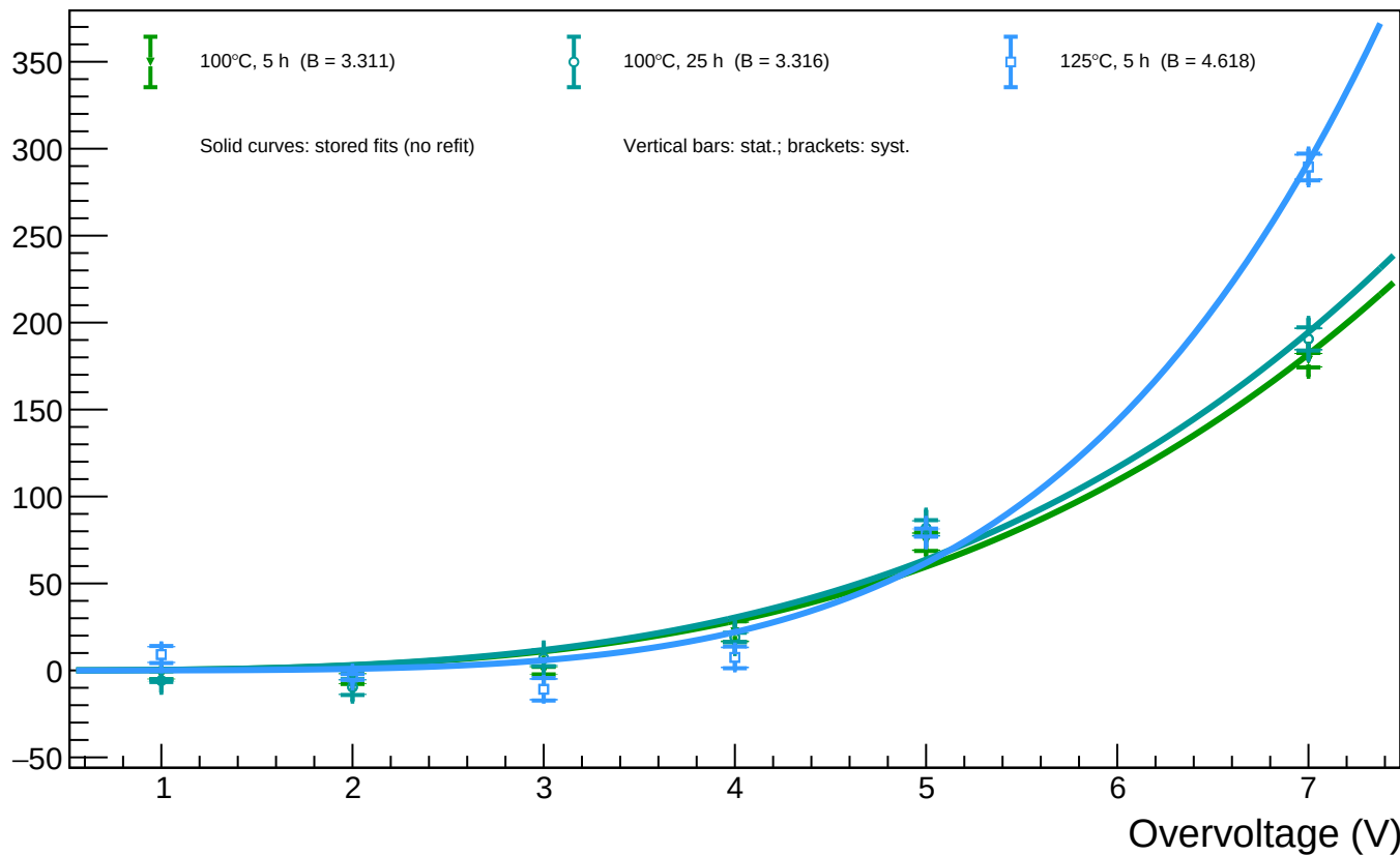
A1_T=20 - Spot 71 (x = 1386.79, y = 117.31): luminosity vs overvoltage for all annealing phases
