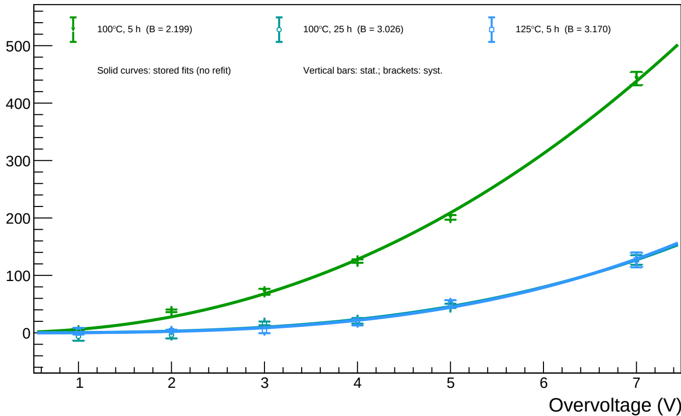
A1_T=20 - Spot 72 (x = 1403.83, y = 206.32): luminosity vs overvoltage for all annealing phases
