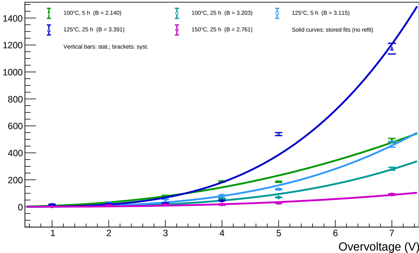
A1_T=20 - Spot 73 (x = 1845.62, y = 888.35): luminosity vs overvoltage for all annealing phases
