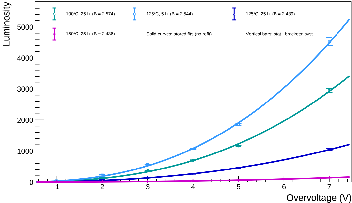
A1_T=20 - Spot 77 (x = 1088.43, y = 521.96): luminosity vs overvoltage for all annealing phases
