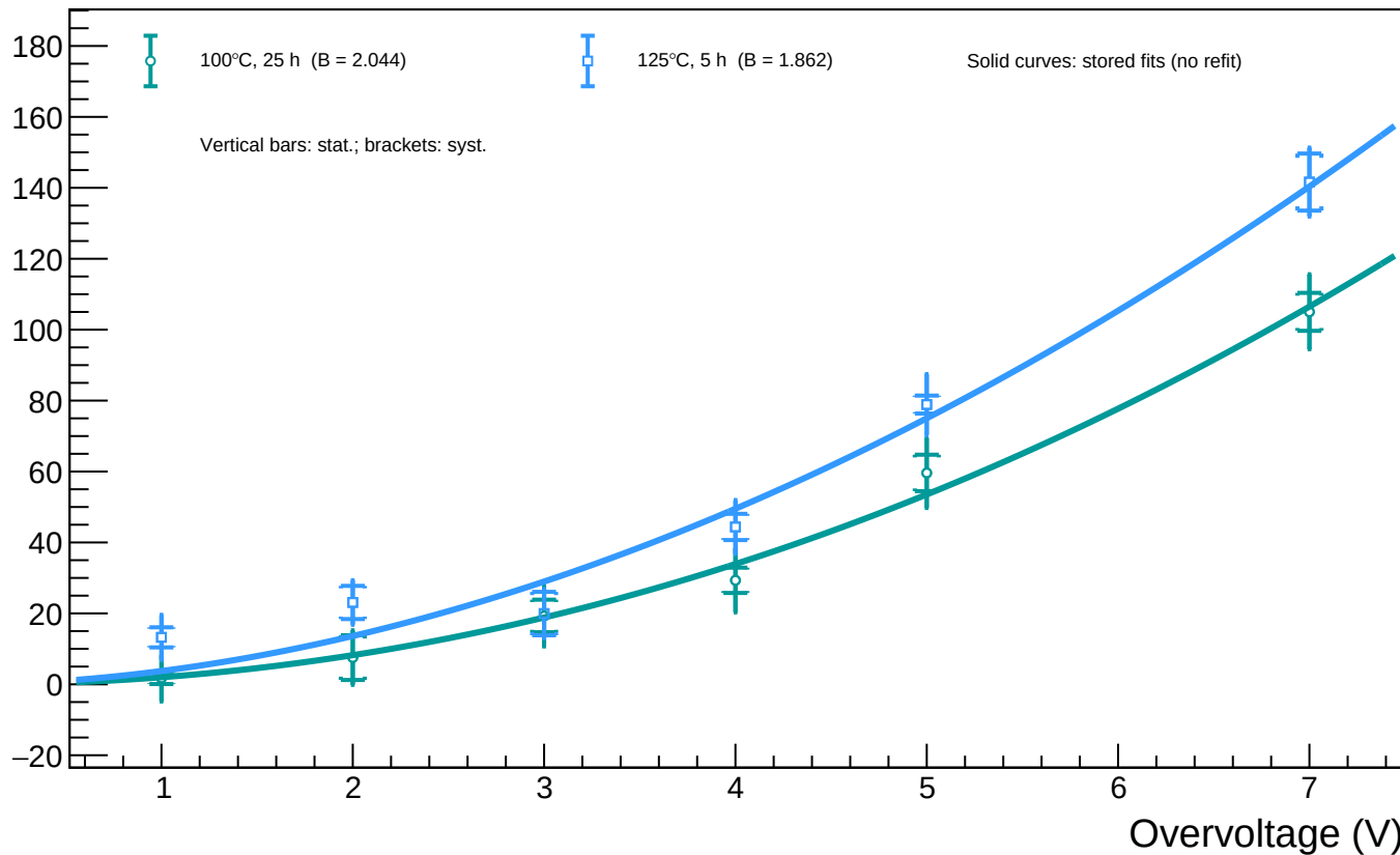
A1_T=20 - Spot 79 (x = 1424.76, y = 351.19): luminosity vs overvoltage for all annealing phases
