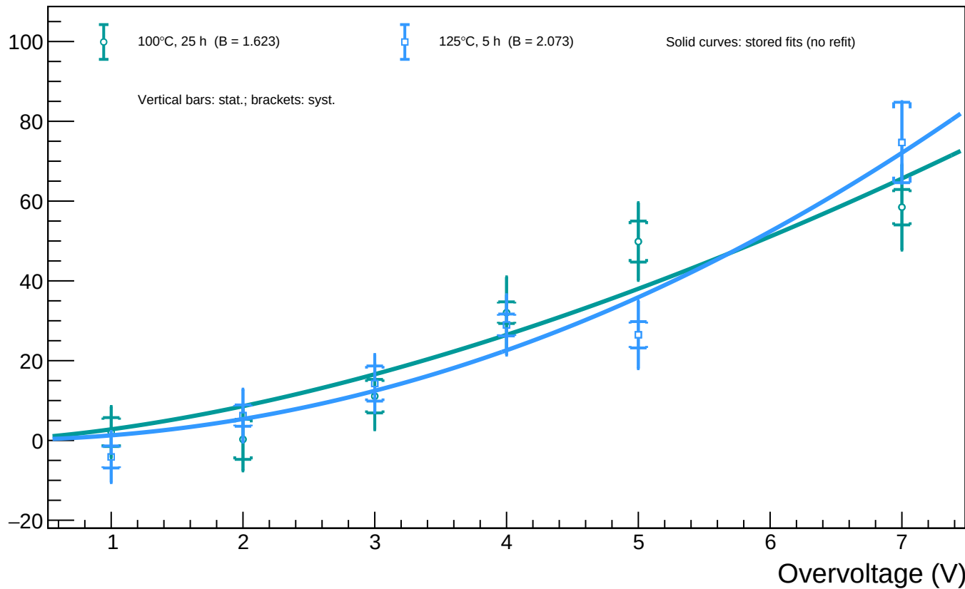
A1_T=20 - Spot 80 (x = 1679.34, y = 253.77): luminosity vs overvoltage for all annealing phases
