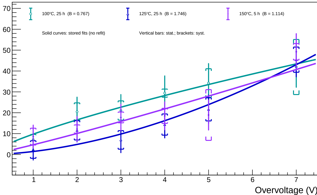
A1_T=20 - Spot 81 (x = 1722.05, y = 805.20): luminosity vs overvoltage for all annealing phases
