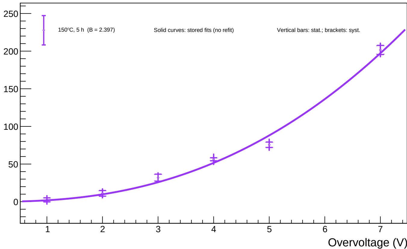
A1_T=20 - Spot 87 (x = 1557.82, y = 208.17): luminosity vs overvoltage for all annealing phases
