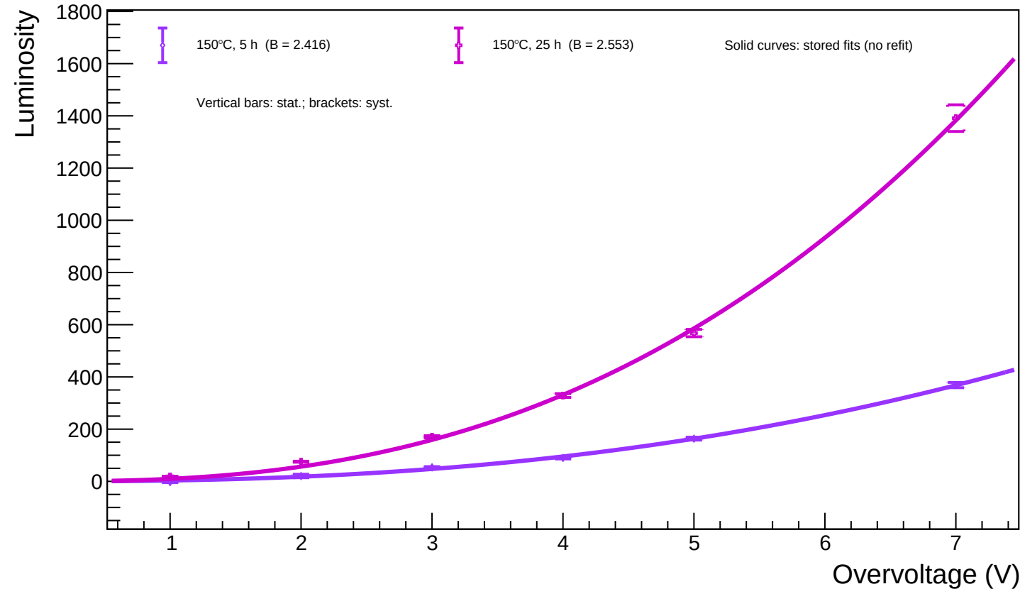
A1_T=20 - Spot 88 (x = 490.61, y = 96.64): luminosity vs overvoltage for all annealing phases
