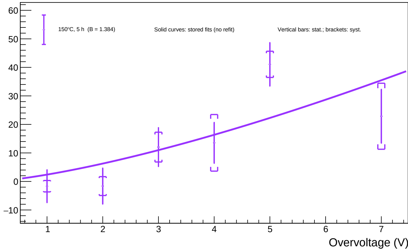
A1_T=20 - Spot 89 ( x = 731.20 , y = 247.34 ): luminosity vs overvoltage for all annealing phases
