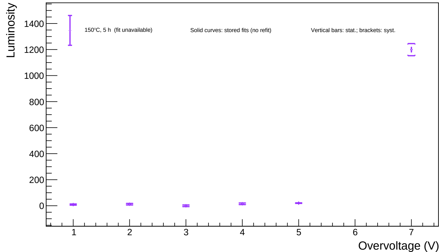
A1_T=20 - Spot 91 (x = 1267.81, y = 787.96): luminosity vs overvoltage for all annealing phases
