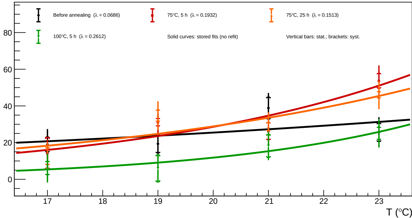
A1_v=5 - Spot 11 (x = 417.46, y = 548.49): luminosity vs temperature for all annealing phases
