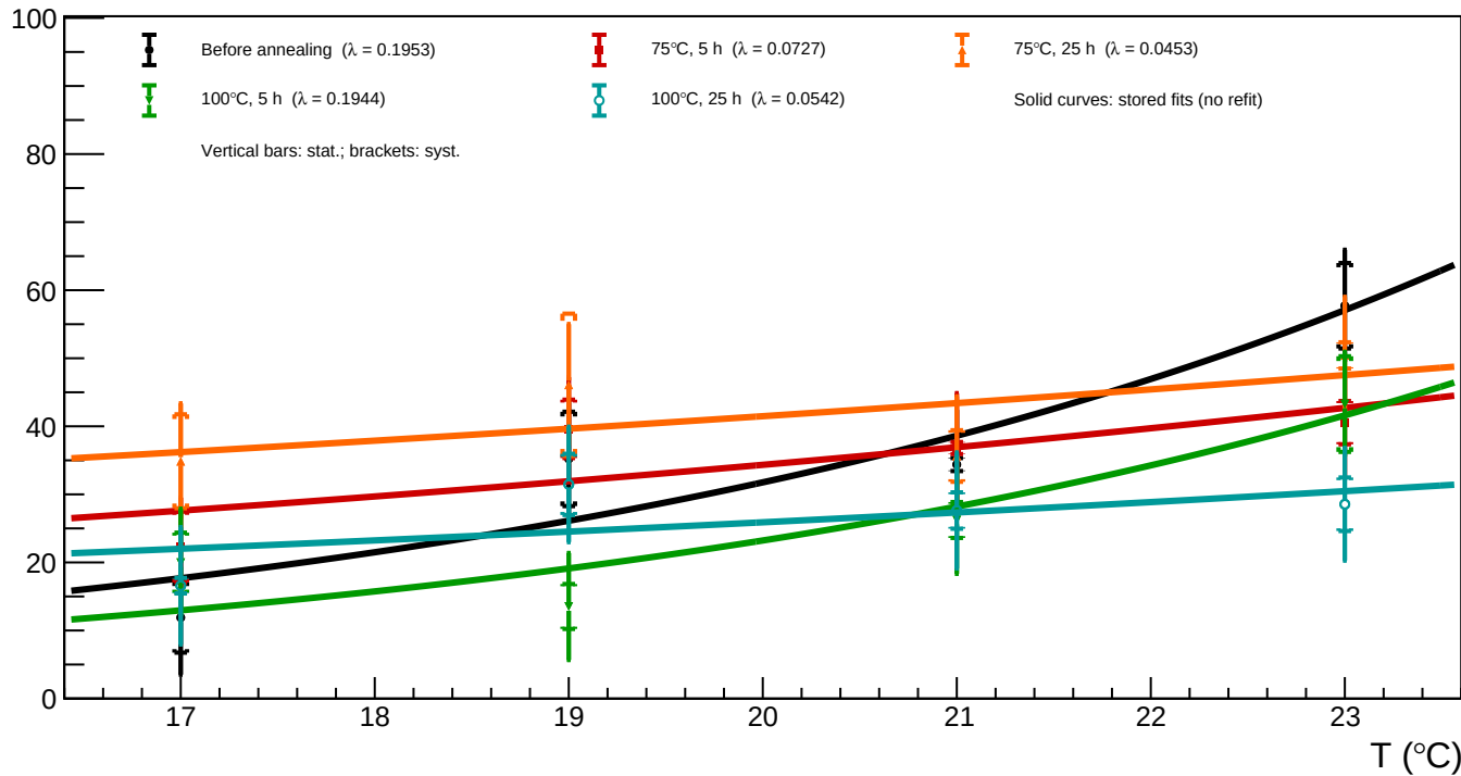
A1_v=5 - Spot 16 (x = 610.10, y = 334.75): luminosity vs temperature for all annealing phases
