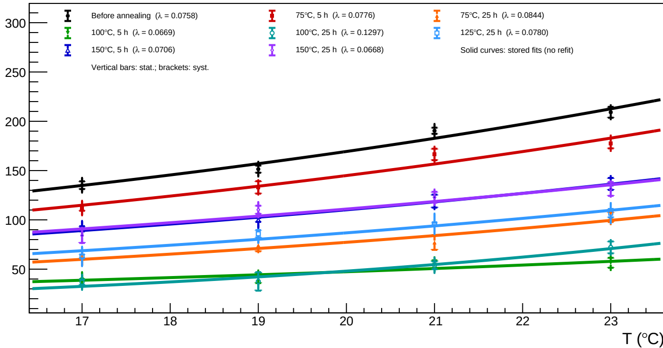
A1_v=5 - Spot 17 (x = 649.54, y = 438.85): luminosity vs temperature for all annealing phases
