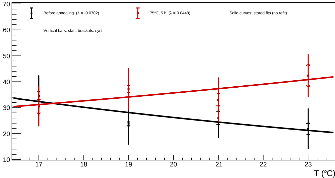
A1_v=5 - Spot 20 (x = 700.57, y = 364.93): luminosity vs temperature for all annealing phases
