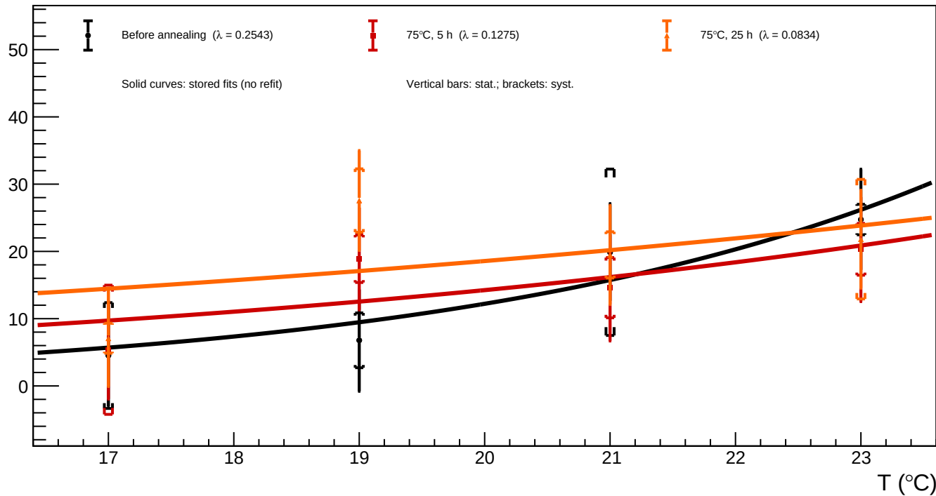
A1_v=5 - Spot 21 (x = 738.81, y = 313.00): luminosity vs temperature for all annealing phases
