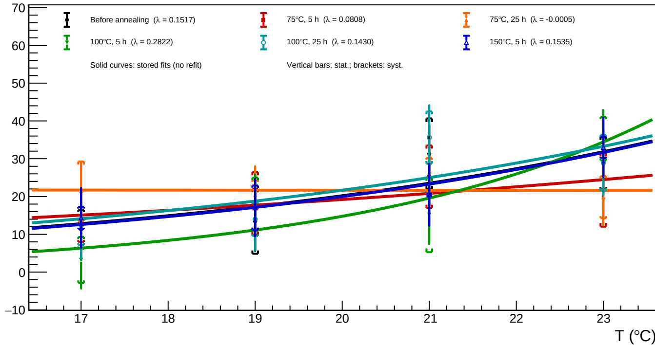
A1_v=5 - Spot 25 (x = 872.22, y = 565.21): luminosity vs temperature for all annealing phases
