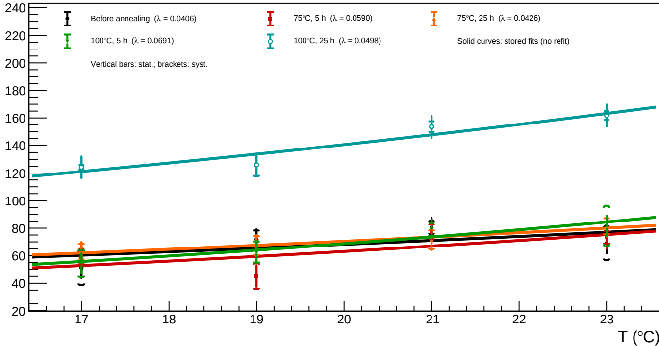
A1_v=5 - Spot 28 (x = 1051.01, y = 803.23): luminosity vs temperature for all annealing phases
