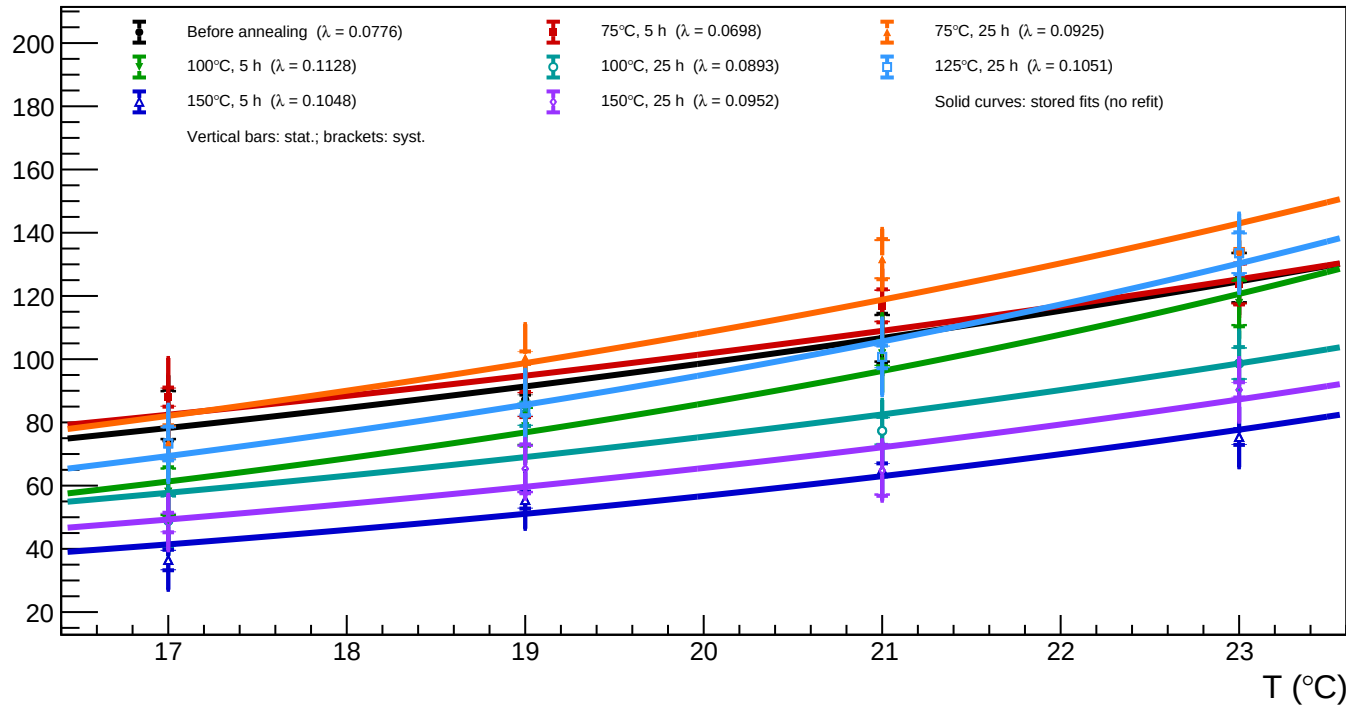
A1_v=5 - Spot 31 ( x = 1088.76 , y = 686.78 ): luminosity vs temperature for all annealing phases
